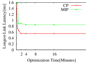
Figure 7: CP vs MIP Convergence: Longest Link (k=20)
