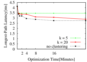
Figure 9: MIP Convergence with k-means: Longest Path
