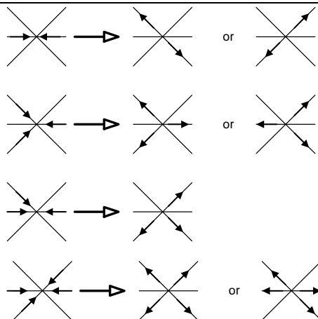
Figure 2 Particle collision rules in the Lattice gas automaton [Orme 95]
