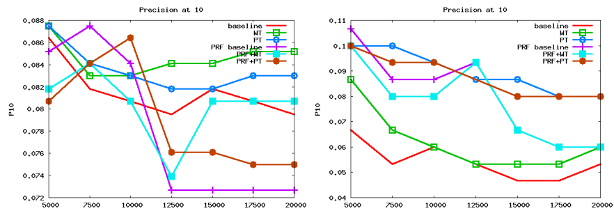
Fig. 3. Dirichlet prior \mu tuning for German (left) and French (right) versus P10 (y axis).
