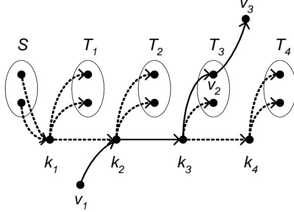
Figure 1: Outfork inequality for R = (k_1, k_2, k_3, k_4) and the path p = (v_1, k_2, k_3, v_2, v_3) . Arcs in the outfork inequality are dashed while arcs in path p are solid. The arcs (k_2, k_3) and (k_3, v_2) are used in both the outfork inequality and in the path p
