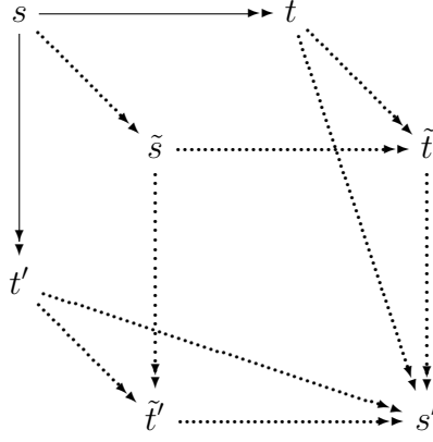
Fig. 2. The proof of Theorem 40.
