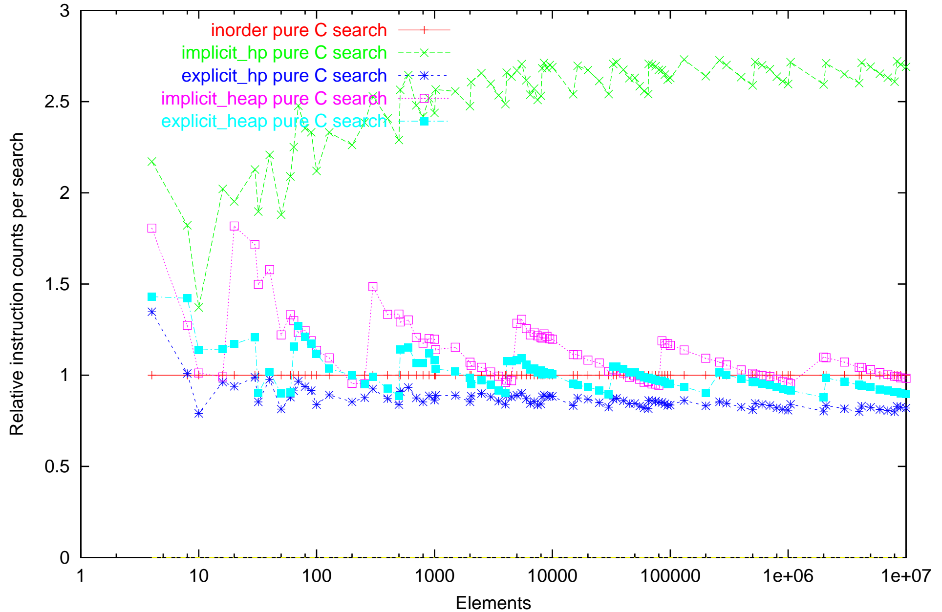
Instruction count of static search on Athlon computer. Dataset: successfull_repetitive_cycle
