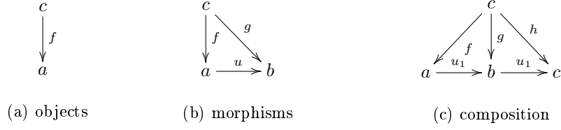
Figure 4.1: Coslice category.
