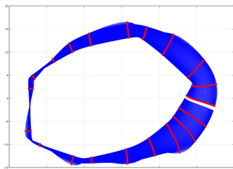
Figure 2.2: Curvature flow, by evolving only the node points of the spline curve. Here the curve is represented by 3^{rd} B-splines, hence the properties of the curve like curvature etc., are accurately computed. But still the evolution takes the node points to lie on a straight line, after which the evolution practically stops. This happens because the curvature information on the entire curve is not taken into account. In our formulation, the projection operator takes into account the curvature information in the neighborhood of the node points, as shown in the previous section
