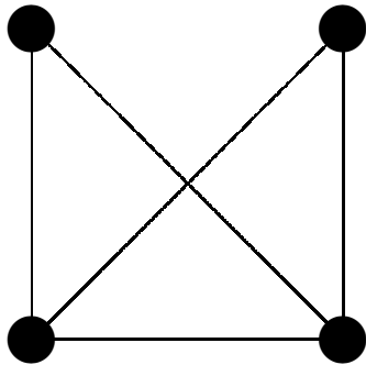
HAM-CYCLE
